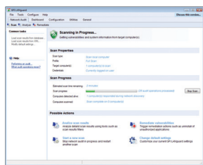
GFI LANguard full scan in progress
